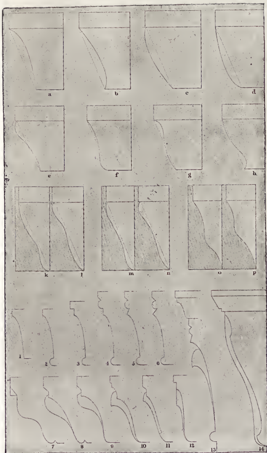
PLATE XV: CORNICE PROFILES
